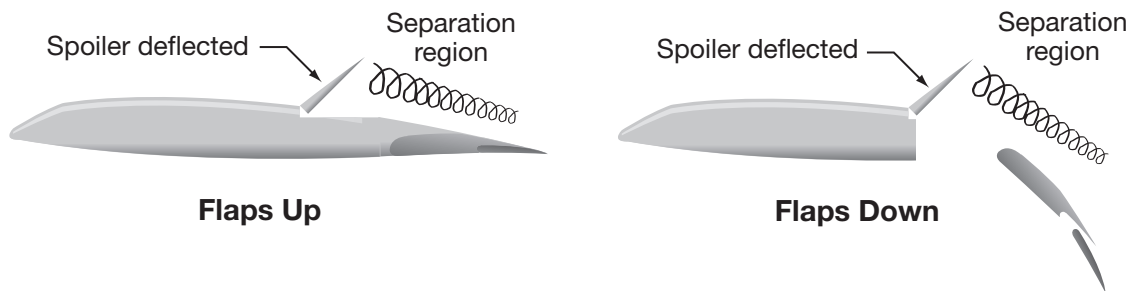
Figure 23 Spoiler Devices
