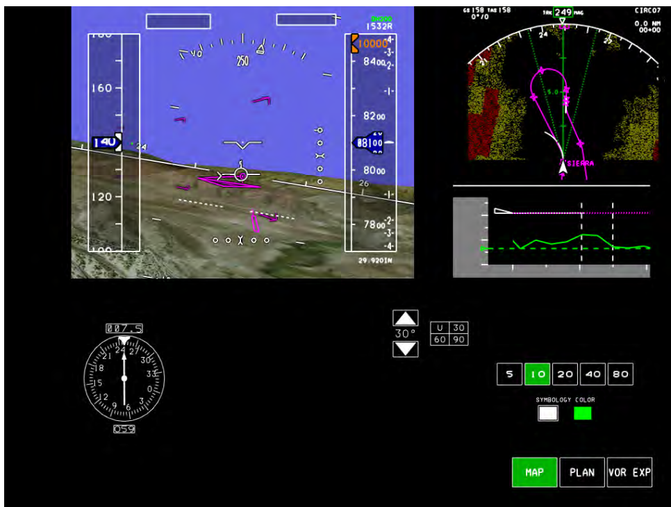
Figure 45. Size X photo-realistic terrain in a left turn.
