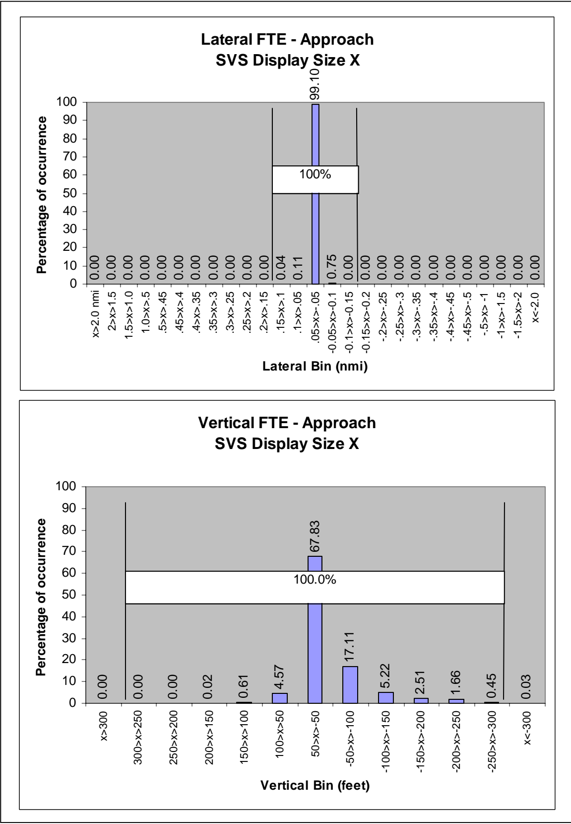
Figure 48. Lateral and Vertical FTE for the SVS Size X display.
