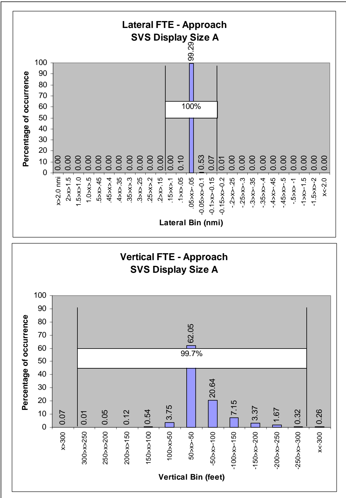
Figure 47. Lateral and Vertical FTE for the SVS Size A display.
