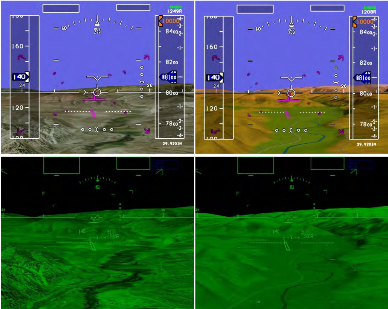
Color photo-realistic (top left), Green photo-realistic for HUD (bottom left), Color generic (top right), Green generic for HUD(bottom right).
