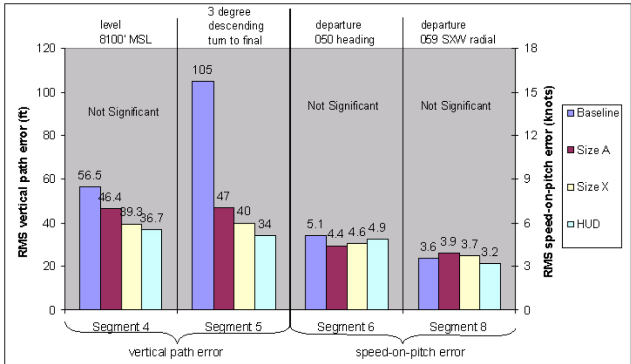
Figure 12. Vertical RMS error for all pilots.
