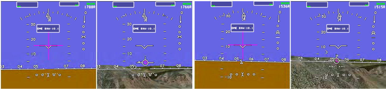
Figure 7. Baseline and SVS displays for nominal run (two left) and baseline and SVS displays for CFIT run (two right)
