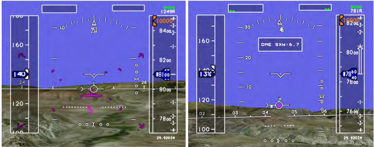
Figure 29. SVS guidance symbology: approach (left) ghost airplane with tunnel and departure (right) integrated single cue guidance (“ball”).
