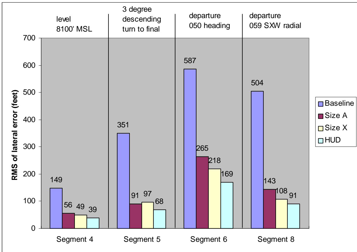
Figure 11. Lateral RMS errors for all pilots by task segment.
