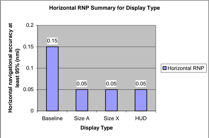
Figure 13. Summary of the approach horizontal RNP for all display types averaged across all subjects.
