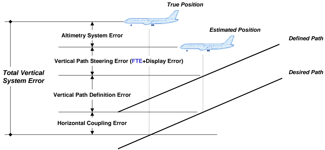
Figure 34. Vertical components of navigation error terms
