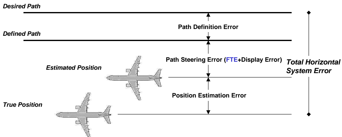
Figure 33. Lateral components of navigation error terms
