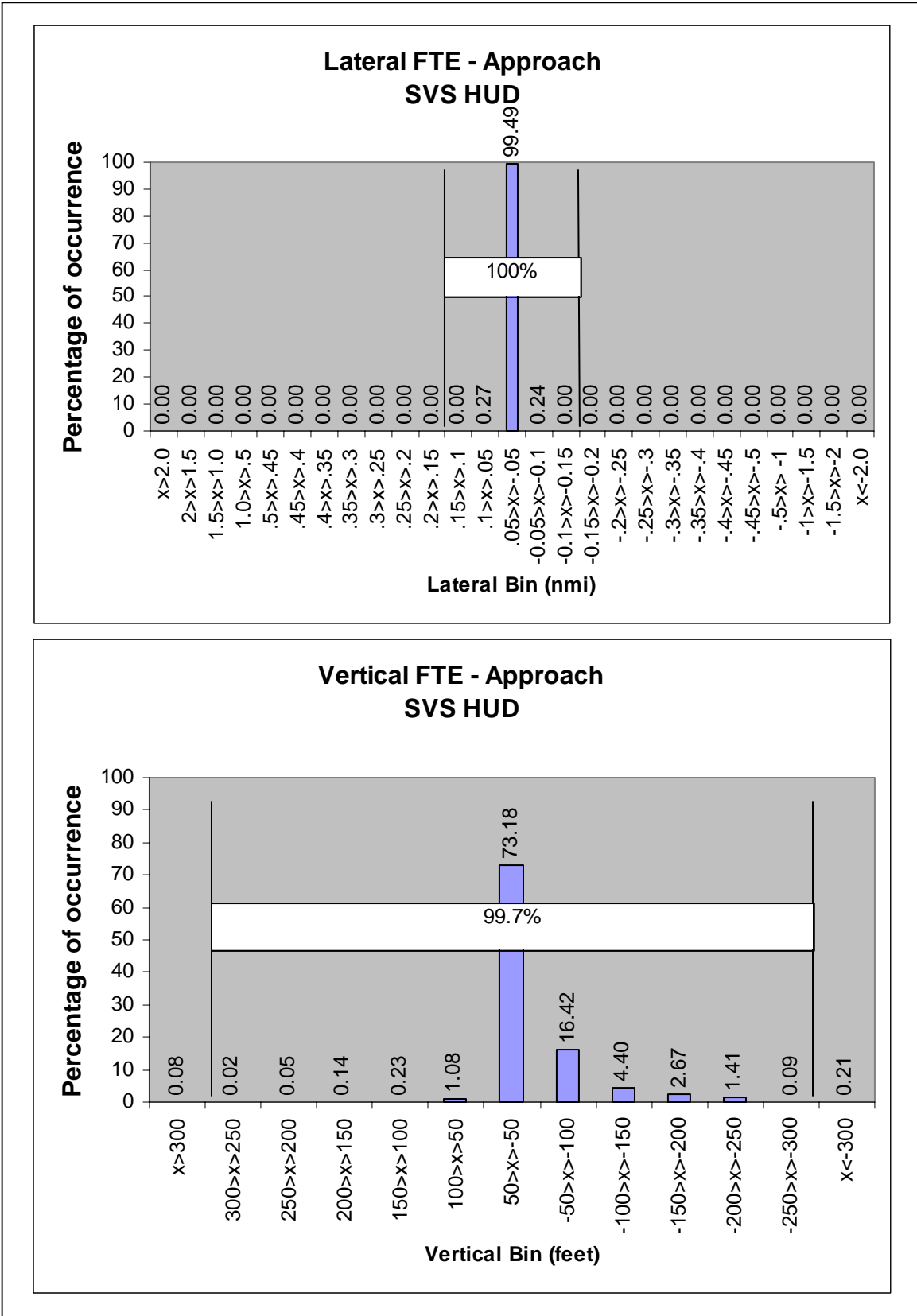
Figure 49. Lateral and Vertical FTE for the SVS HUD.
