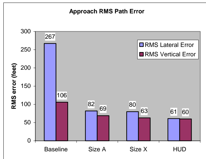
Figure 9. Entire approach path performance errors for display concepts without texturing effects.
