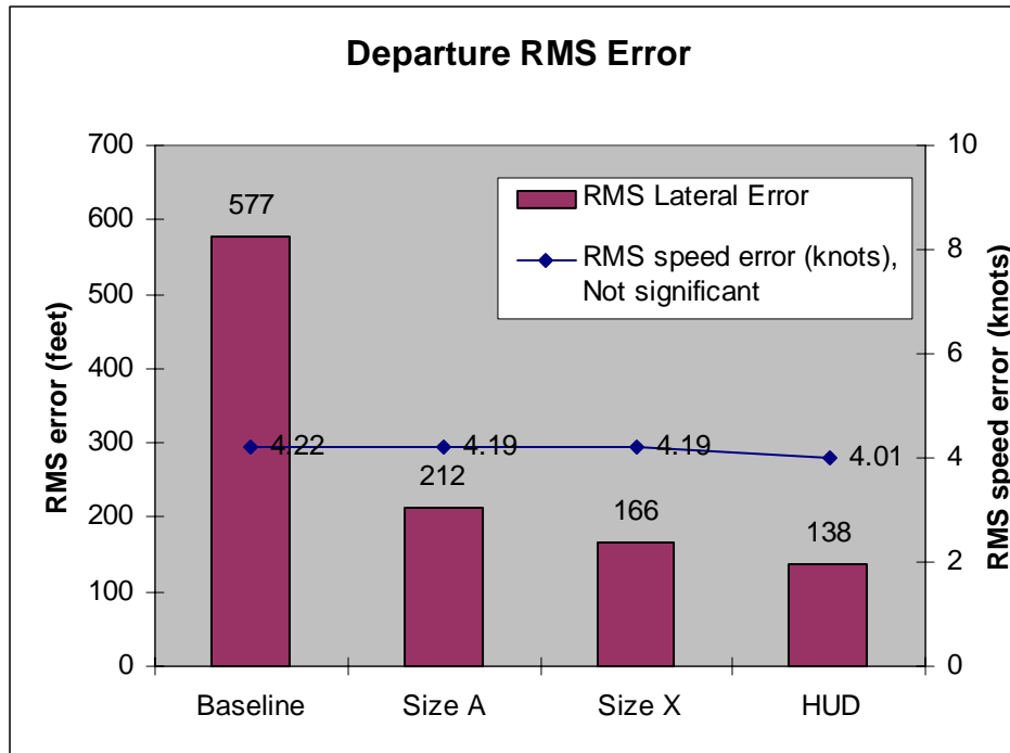
Figure 10. Entire departure path performance errors for display concepts without texturing effects.
