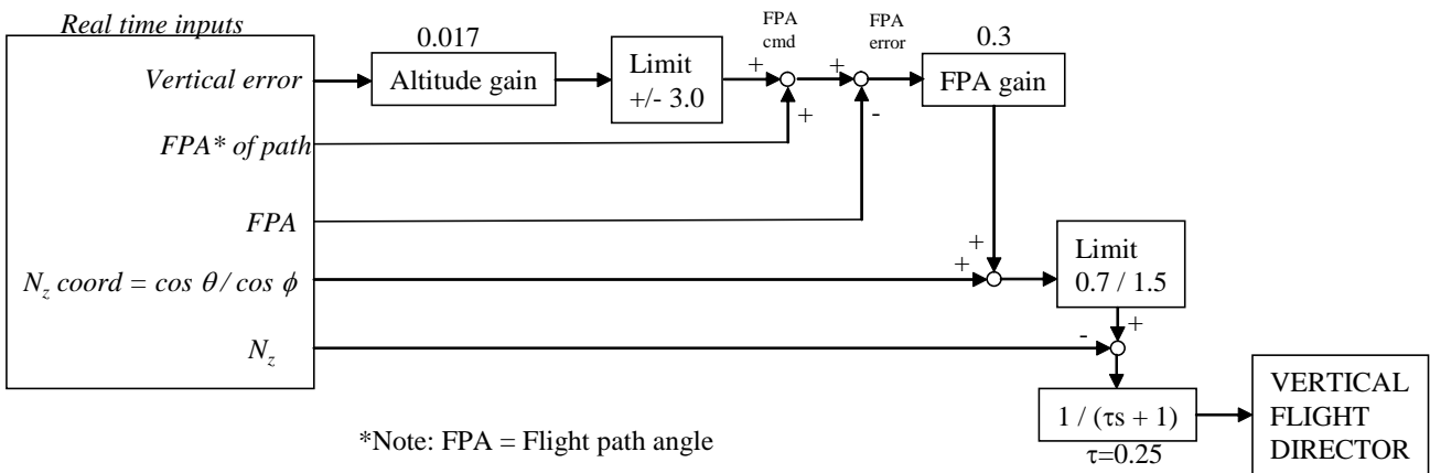
Figure 31. Vertical flight director for the baseline concept approach task.
