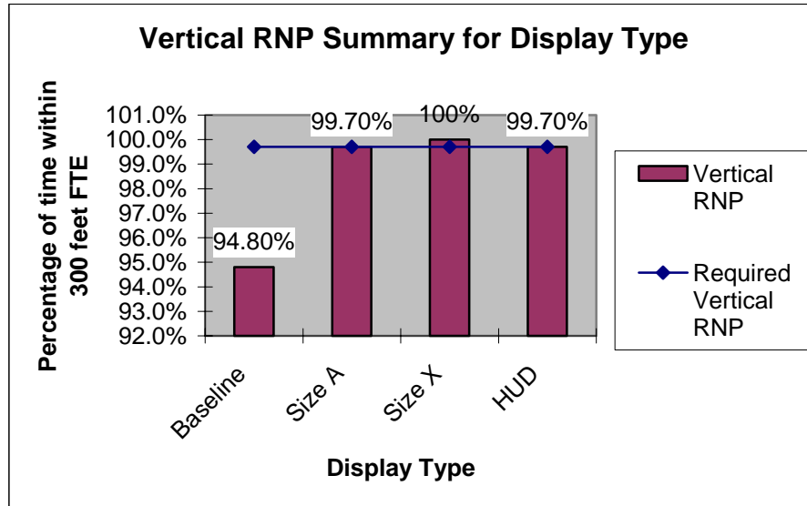
Figure 14. Summary of approach vertical RNP for all display types averaged across all subjects.
