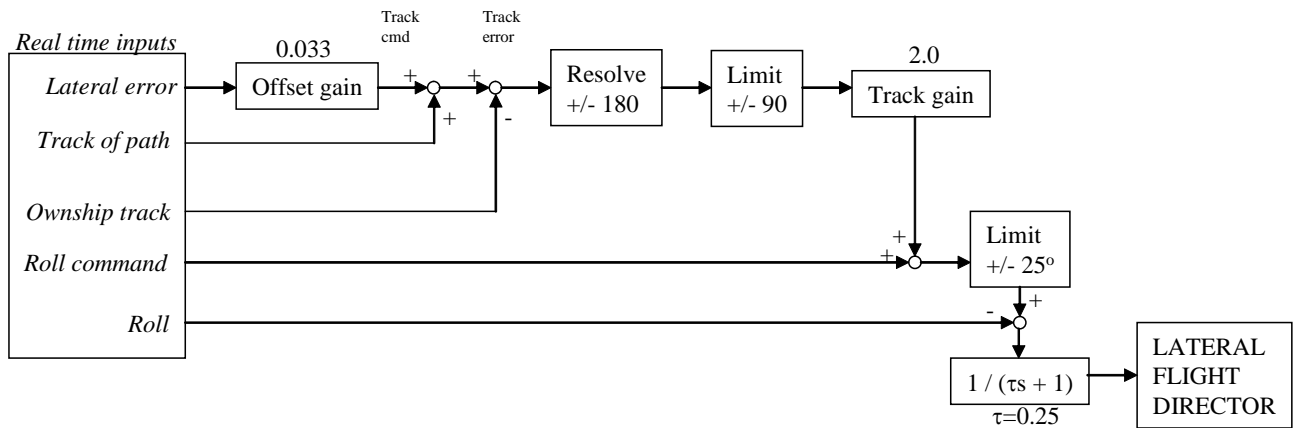
Figure 30. Lateral flight director for baseline concept approach tasks and for baseline and SVS concepts departure tasks.
