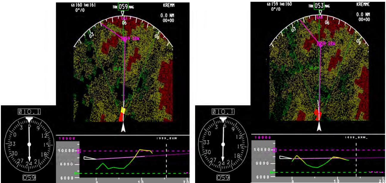
Figure 8. TAWS, VSD and RMI for nominal run (left) and CFIT run (right)
