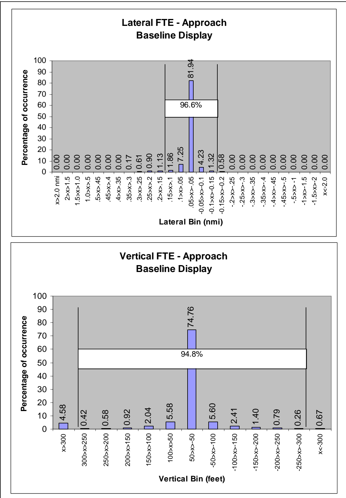
Figure 46. Lateral and Vertical FTE for the baseline display.
