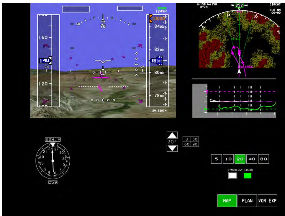
Figure 41. Size X with photo-realistic textured terrain.
