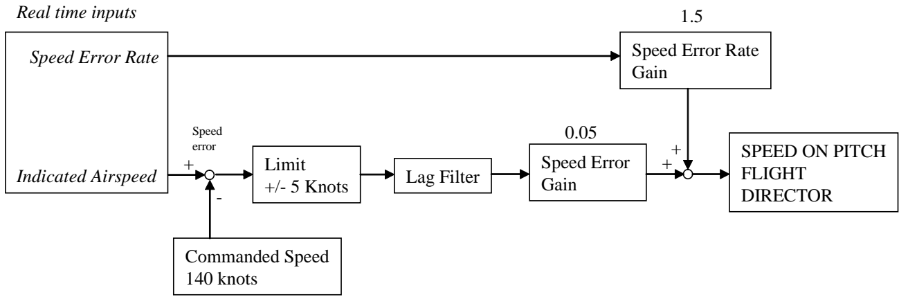
Figure 32. Speed-on-pitch flight director for all display concepts departure tasks.
