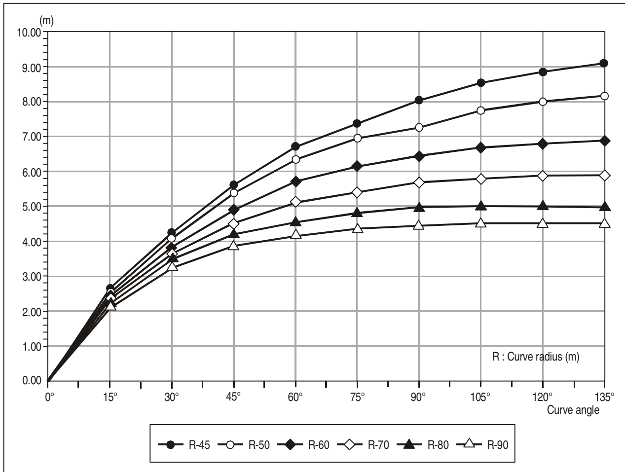
Figure 1-11. Maximum wing tip track-in as a function of curve radius 'R' and curve angle for A330-300 / A340-300
