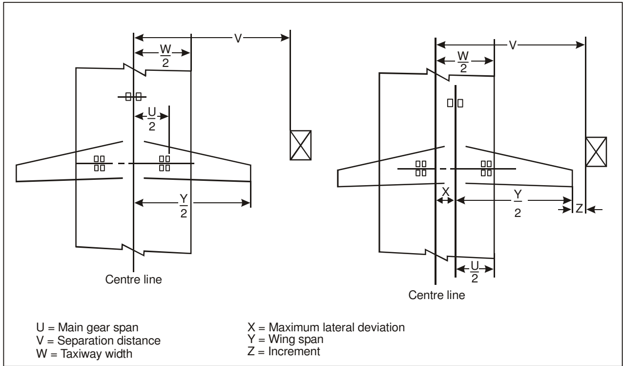
Figure 1-4. Separation distance to an object
