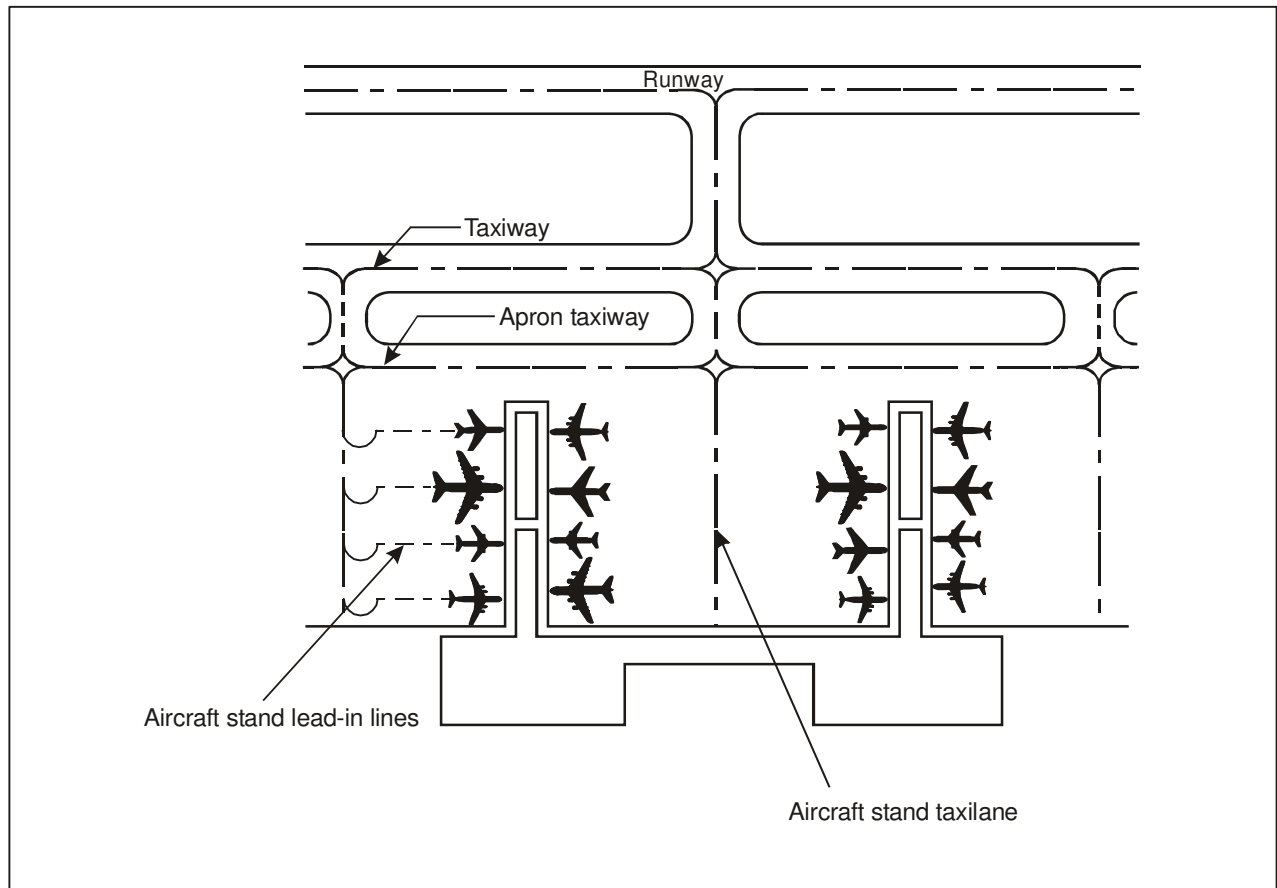
Figure 1-1. Taxiways on aprons
