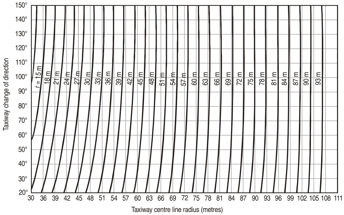
Graph A — Radius of fillet arc (r)
