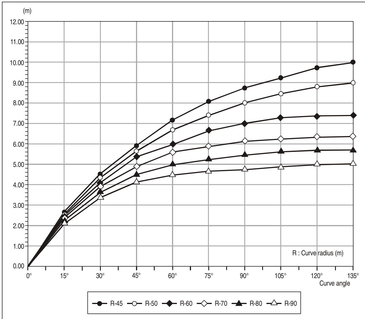
Figure 1-8. Maximum wing tip track-in as a function of curve radius ‘R’ and curve angle for MD11
