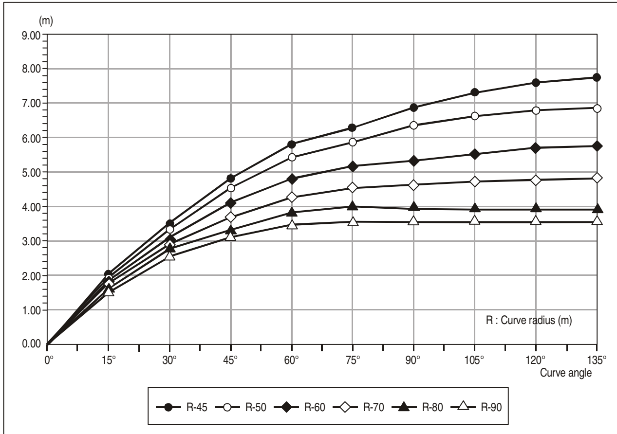
Figure 1-10. Maximum wing tip track-in as a function of curve radius 'R' and curve angle for B747-200
