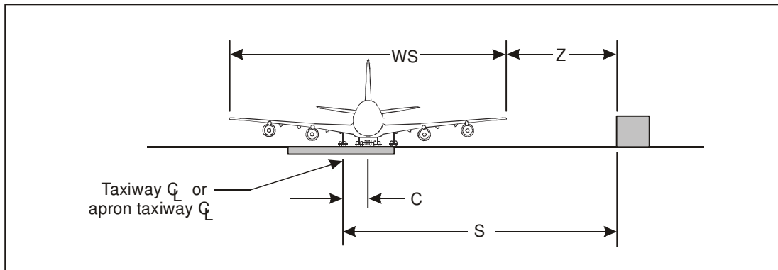
Figure 1-21. Taxiway/apron taxiway-to-object geometry
