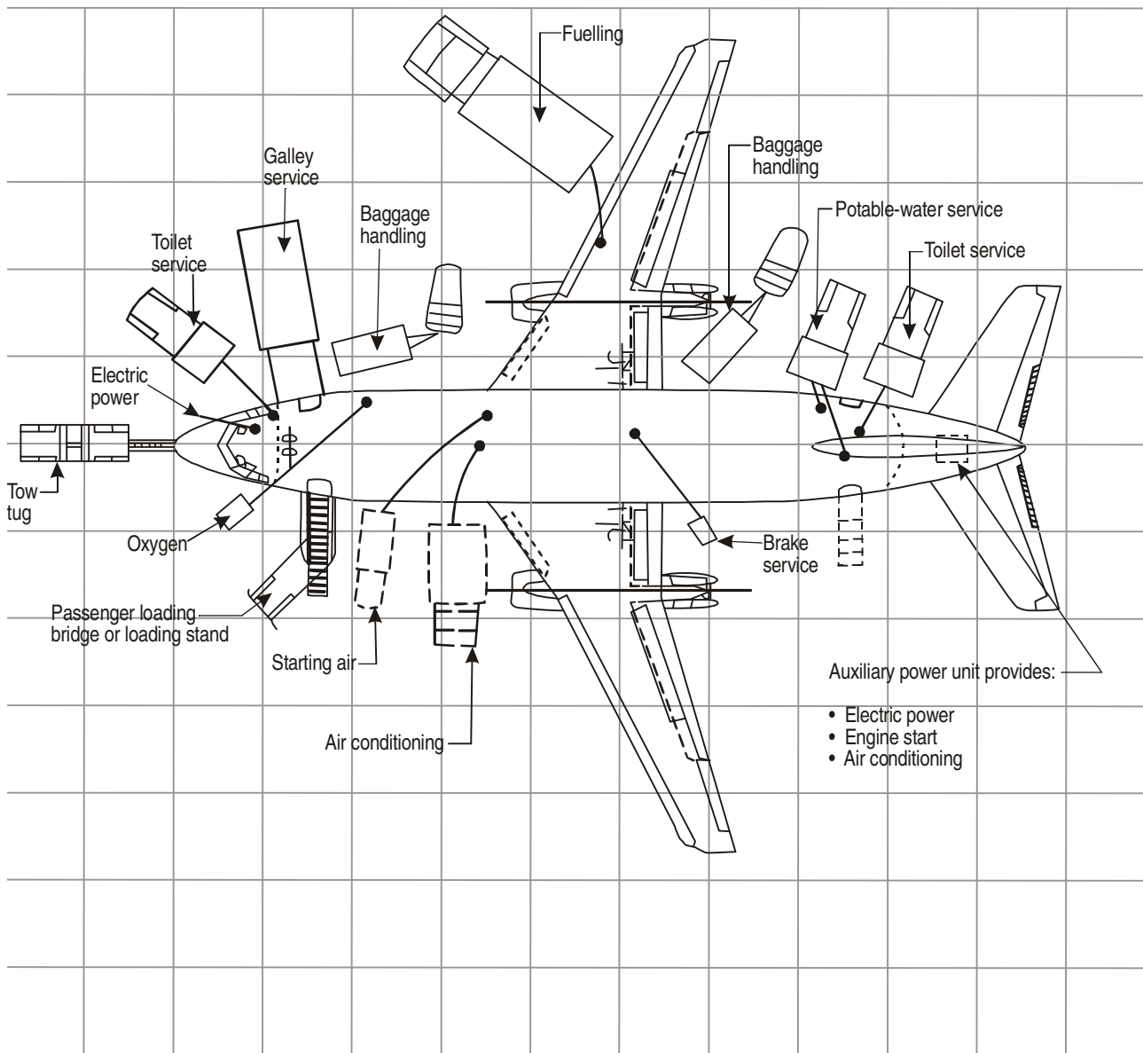
Figure 3-5. Typical ground equipment service layout
