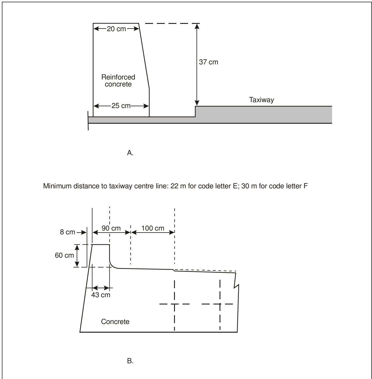
Figure 1-17. Examples of concrete curbs
