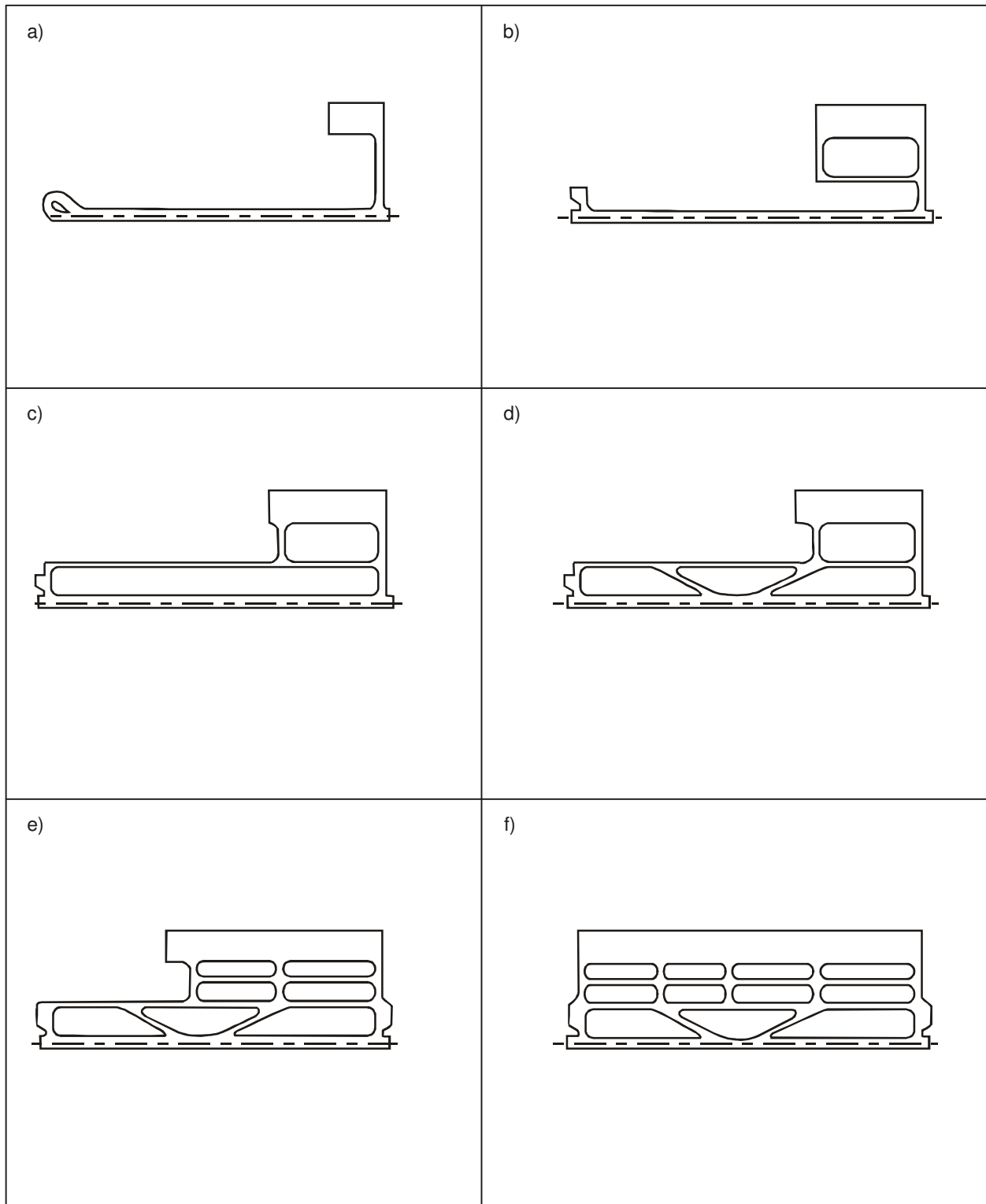
Figure 1-2. Stages in taxiway system development
