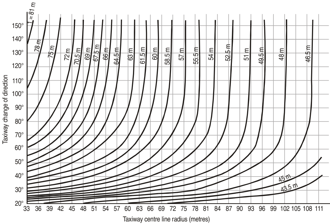
Figure A1-20. Quick reference graph for Boeing 747 (cockpit over taxiway centre line)
