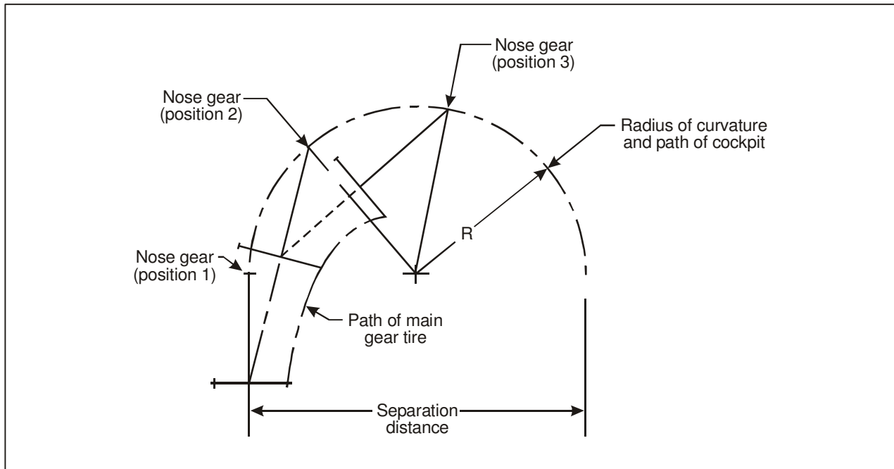
Figure 1-5. Graphical solution of a 180^\circ turn
