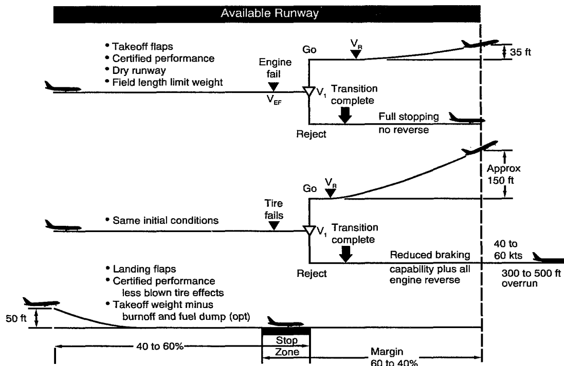
Figure 18 Margin Associated with continuing or rejected takeoff with a tire failure
