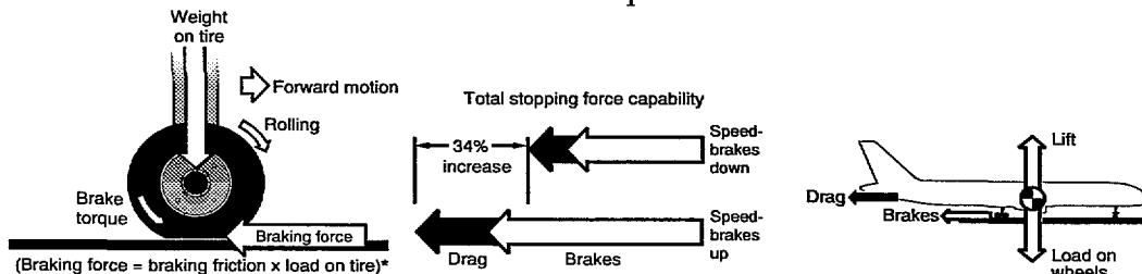
Figure 19 Effect of speedbrakes on the stopping capability of a typical mid-size two engine transport
