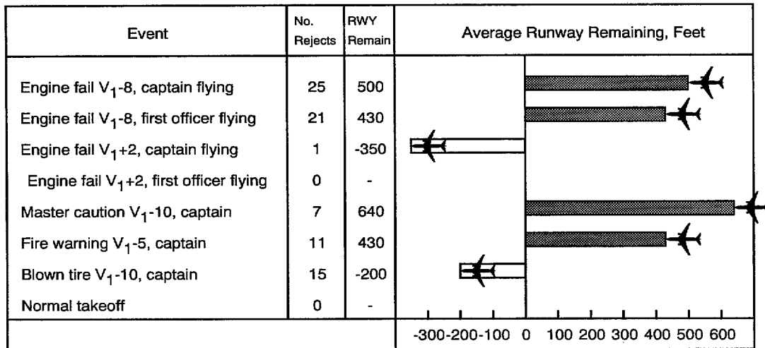
Figure 7 Stopping Performance
