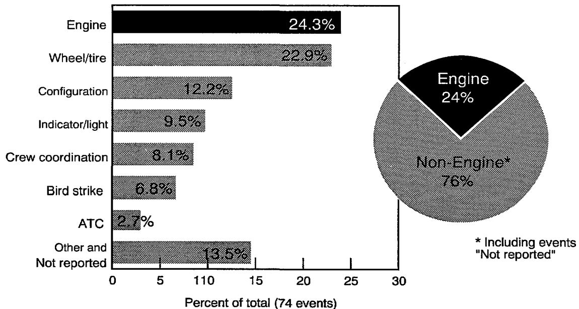
Figure 5 Reasons for initiating the RTO (74 accident/ incident events)
