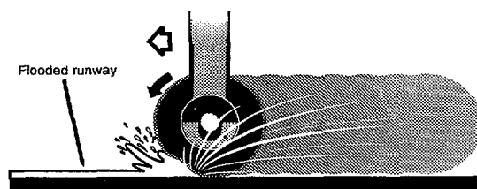
Dynamic Hydroplaning
