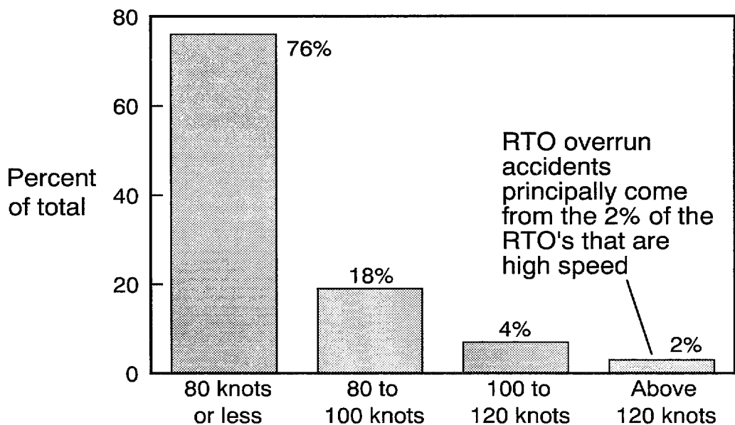
Figure 2 Distribution of RTO Initiation Speeds
