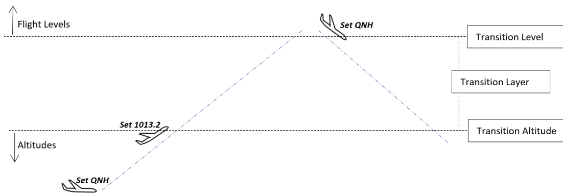
Figure 5 – Transition Altitude/Level
