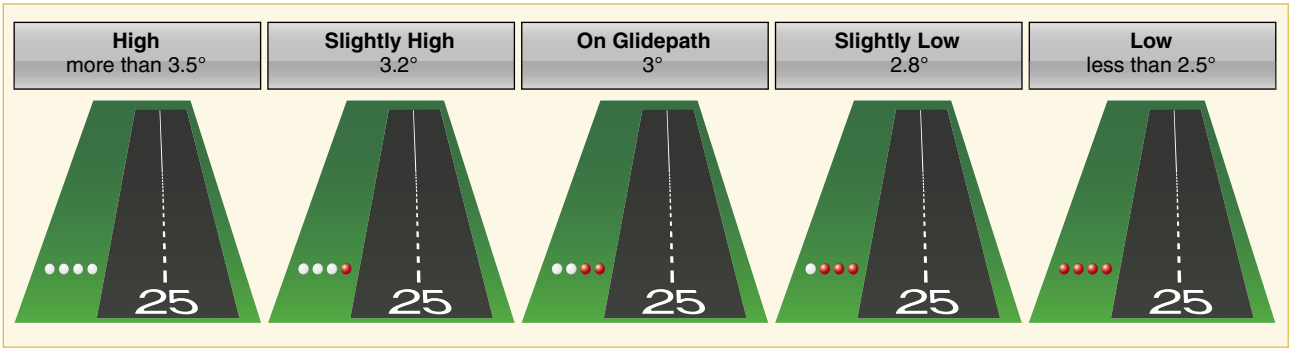
Figure 13-8. Precision approach path indicator.
