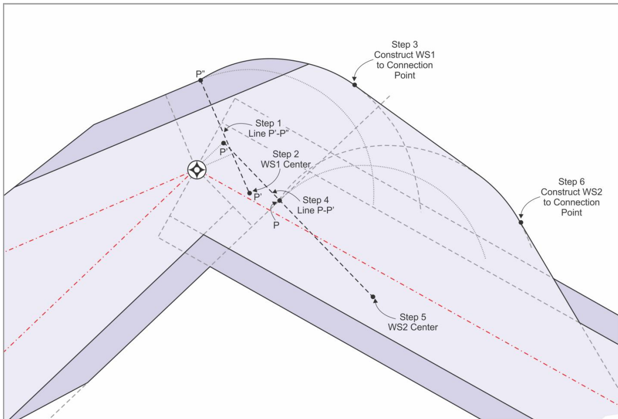
Figure 5-3-21. Late/Outside Turn, Second Turn, FO fix
