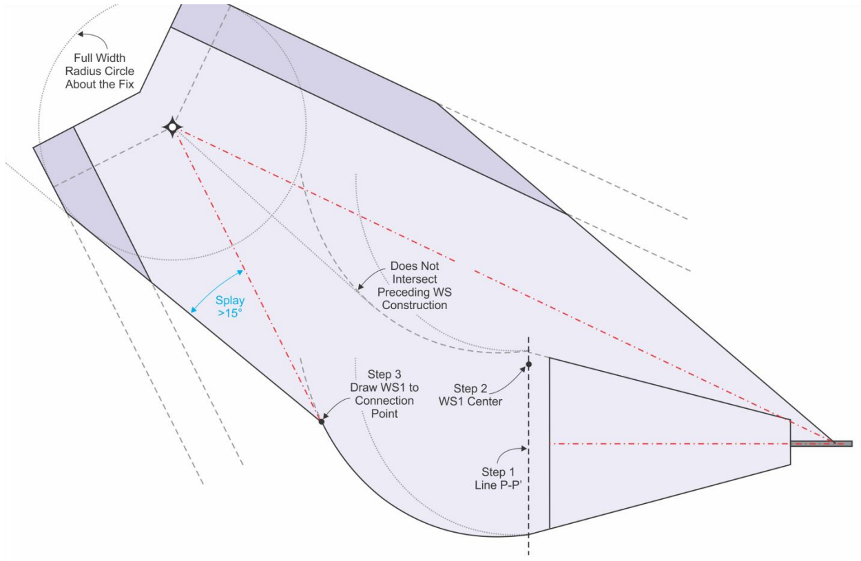
Figure 5-3-17. Late/Outside Turn, First Turn, Case 1, Turn-at-Altitude or FO fix with 1 WS
