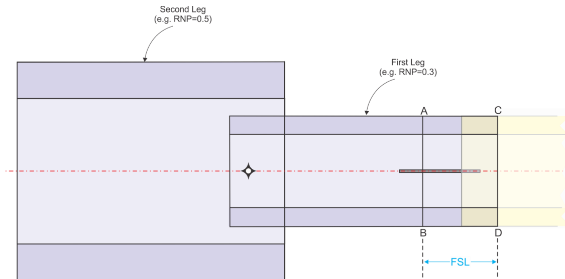
Figure 3-7-1. A-RNP Reduced XTT Area
