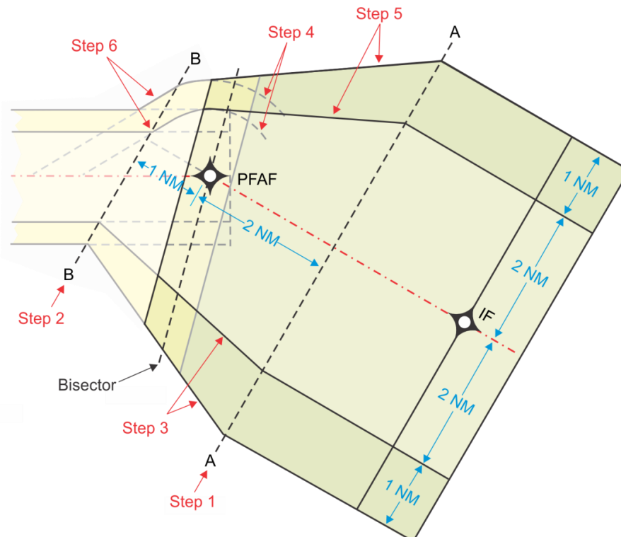
Figure 3-1-5. Offset Intermediate, Example LNAV
