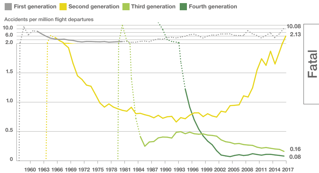
10 year moving average fatal accident rate by aircraft generation
