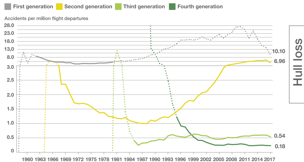
10 year moving average hull-loss rate by aircraft generation
