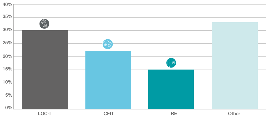
Percentage of fatal accidents by accident category 1998-2017
