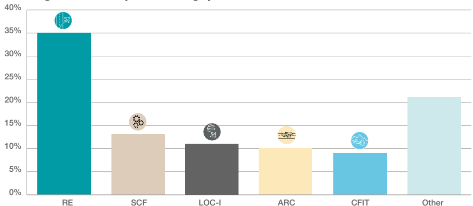
Percentage of hull losses by accident category 1998-2017
