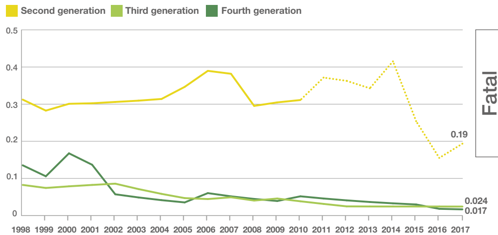
10 year moving average CFIT rate by aircraft generation per million flights
