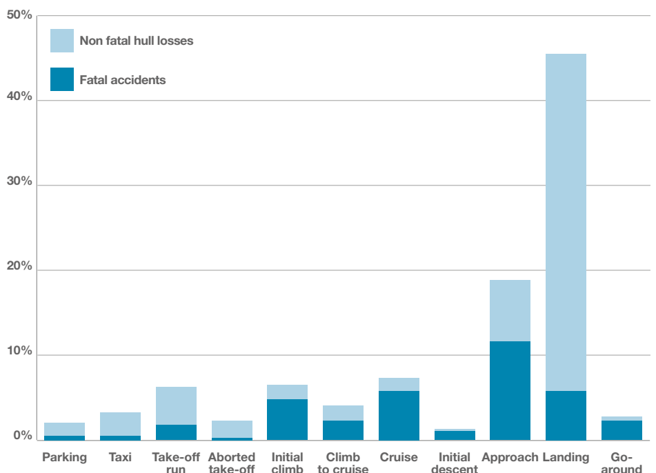
Accidents by flight phase as a percentage of all accidents 1998-2017
