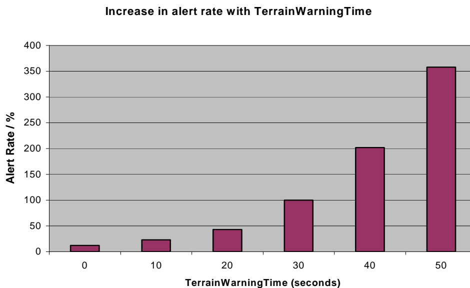
Figure 4-2 Increase in alert rate with TerrainWarningTime (relative to 30seconds rate)
