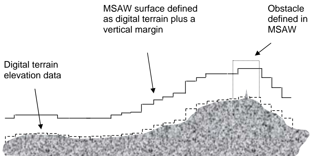
Figure 2-3 Typical MSAW surface defined using digital terrain data with a vertical margin added and supplemented by obstacles.
