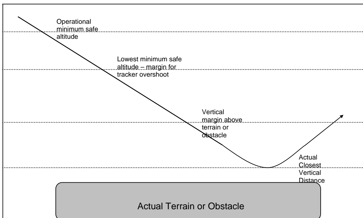
Figure 5-3 Example Points of Risk for MSAW
