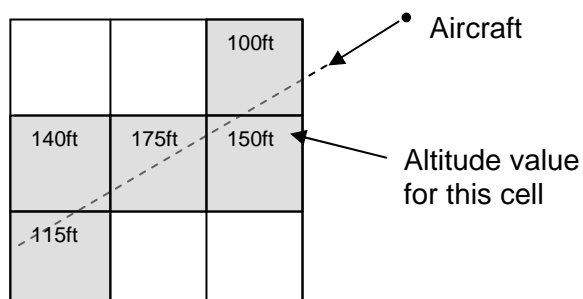
Figure 2-6 Predicted lateral path through the MSAW terrain grid
