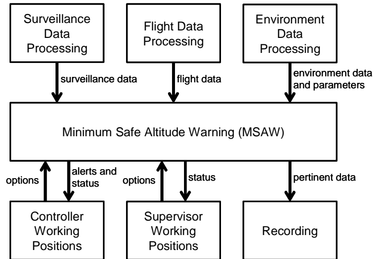
Figure 2-1 MSAW Context Diagram
