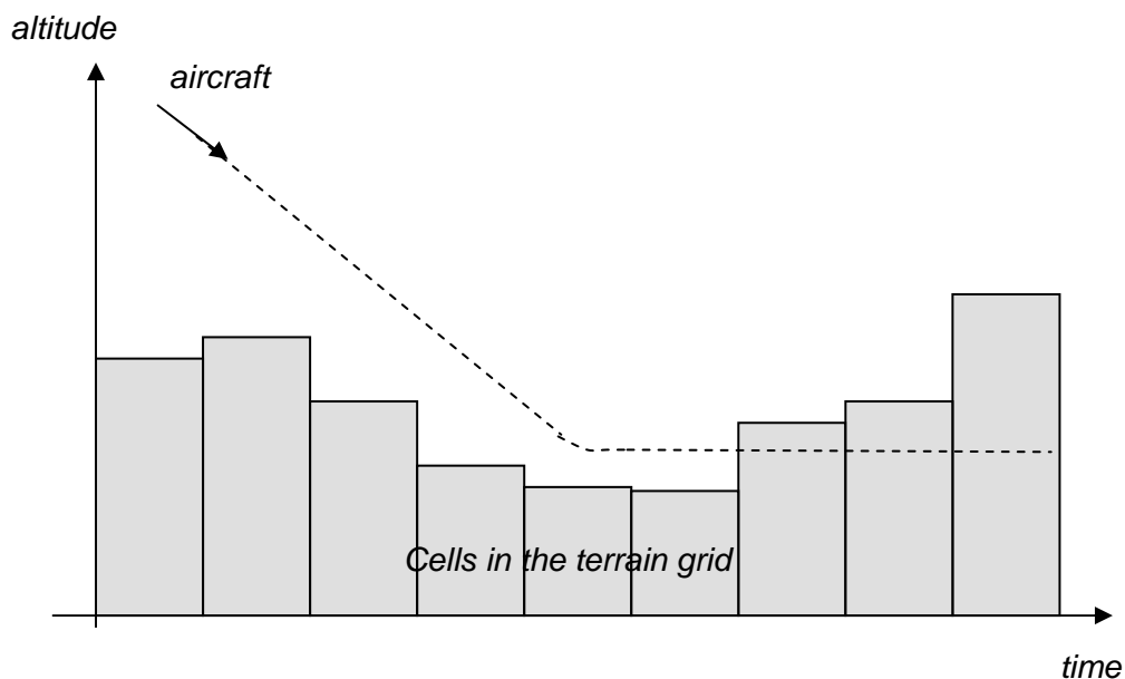
Figure 2-9 Vertical prediction with a level off assumption
