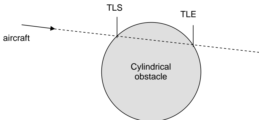
Figure 2-11 Predicted lateral violation of an obstacle
