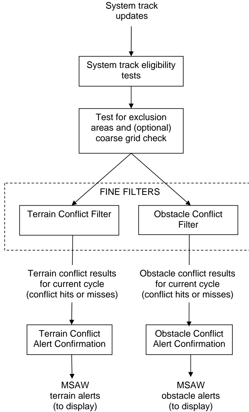
Figure 2-5 MSAW Processing Stages
