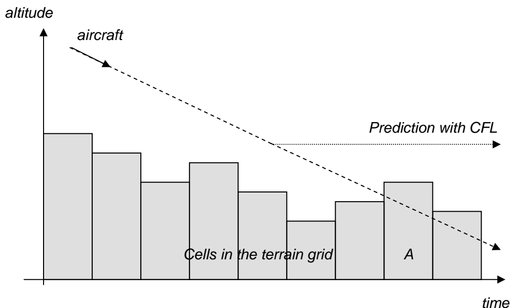
Figure 2-7 Vertical prediction with the CFL
