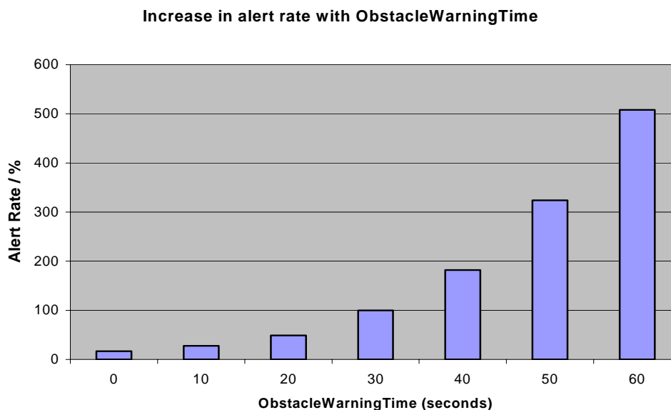
Figure 4-5 Increase in alert rate with ObstacleWarningTime (relative to 30seconds rate)
