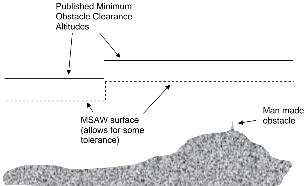
Figure 2-2 Typical MSAW surface defined using polygons
