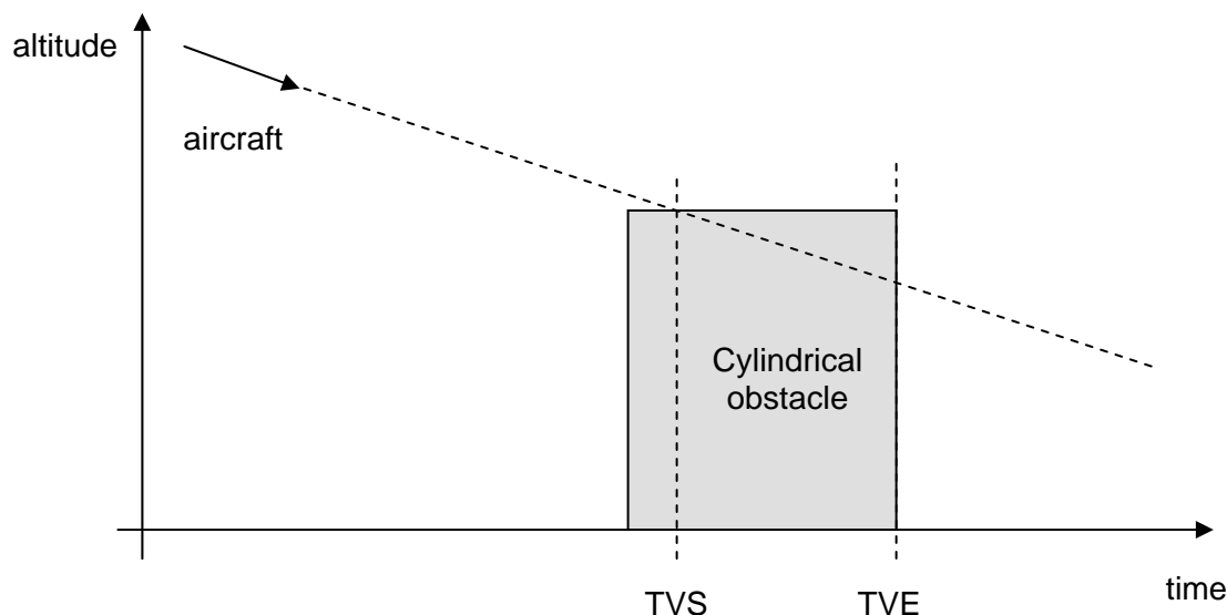
Figure 2-12 Predicted vertical violation of an obstacle
