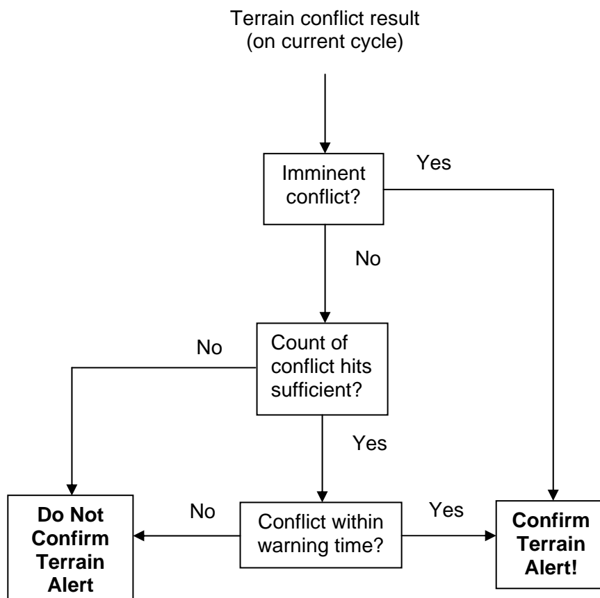
Figure 2-15 Alert confirmation stage for the terrain conflict filter
