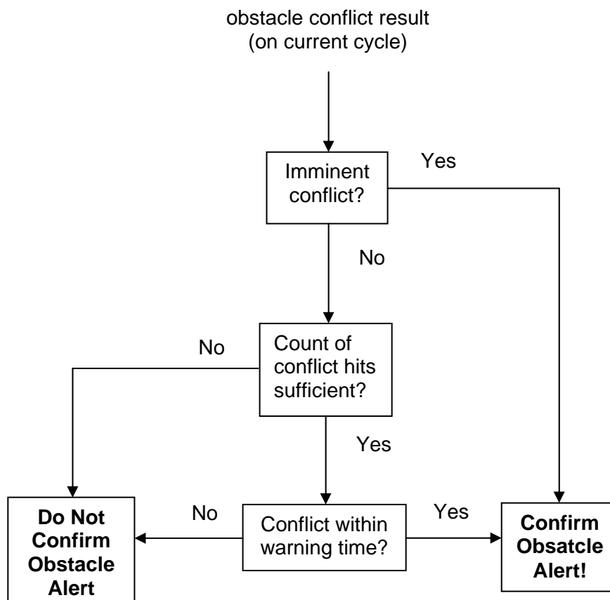
Figure 2-17 Alert confirmation stage for the obstacle conflict filter
