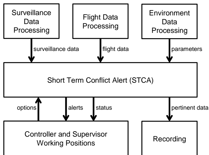
Fig. 3: STCA Context Diagram
