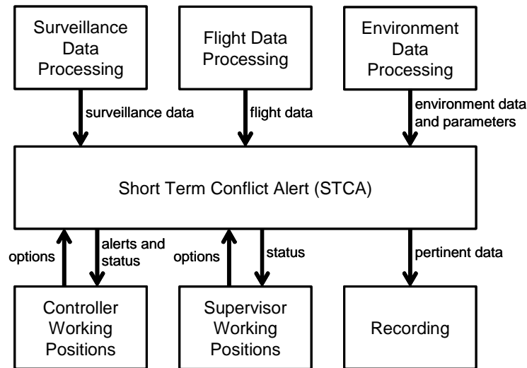
Figure 3-2: STCA Context Diagram
