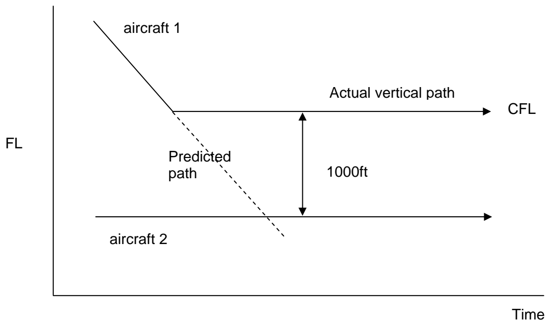
Figure 3-3 The Level-off Situation
