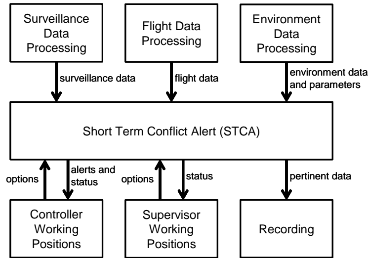
Figure 2-1: STCA Context Diagram
