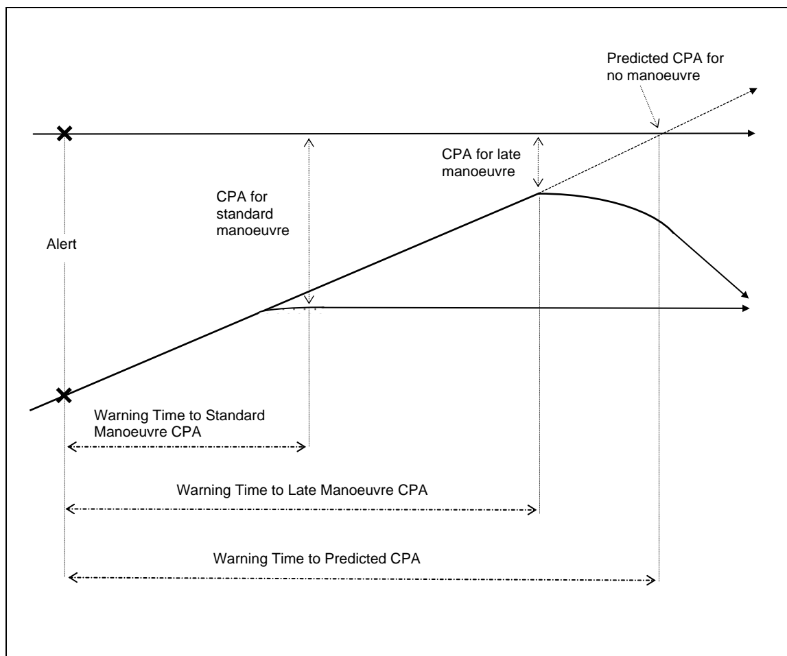
Figure 4-4 Examples of Warning Time Variation
