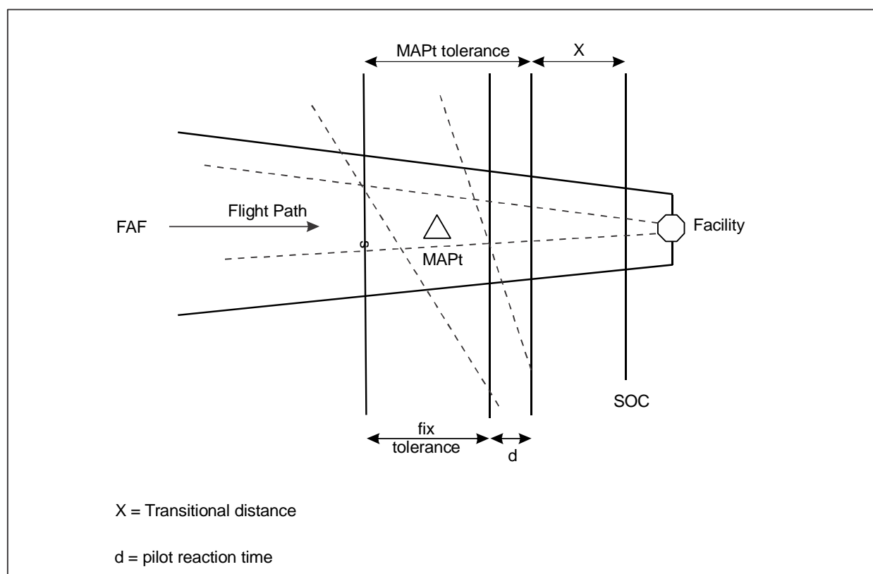
Figure I-4-6-1. Determining SOC with an MAPt defined by a navigation facility or fix
