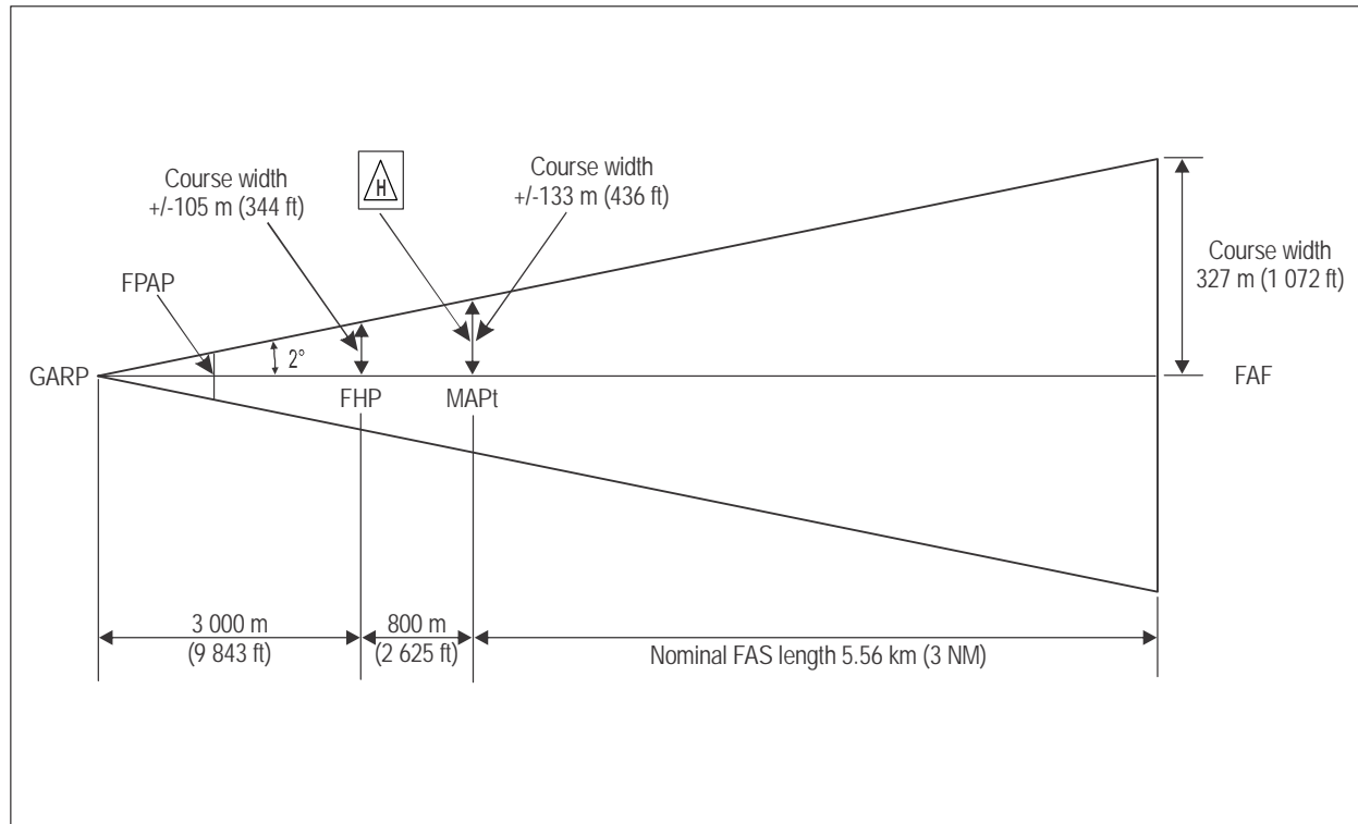
Figure IV-3-App-1. Fictitious helipoint orientation and lateral display scaling
