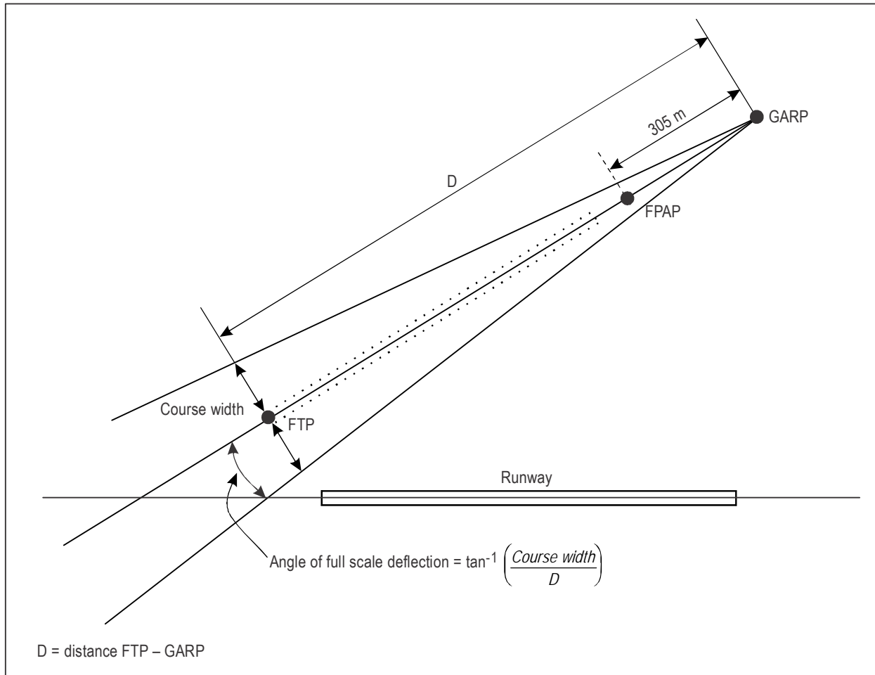
Figure III-3-6-20. GLS Cat I with offset azimuth final approach course alignment
