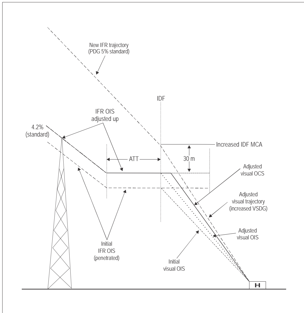
Figure IV-1-4. Mitigation of obstacle penetration in the instrument segment by increasing the IDF MCA
