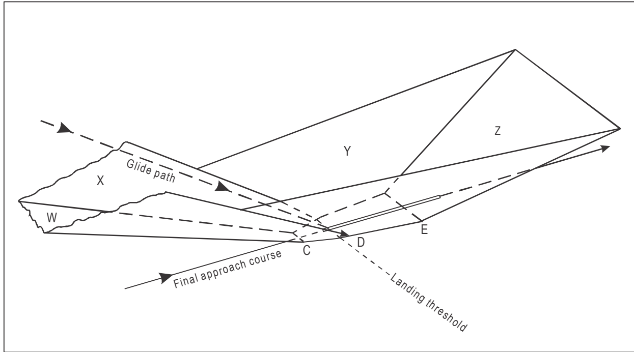
Figure III-3-6-10. Illustration of ILS obstacle assessment surfaces for GLS operations — perspective view
