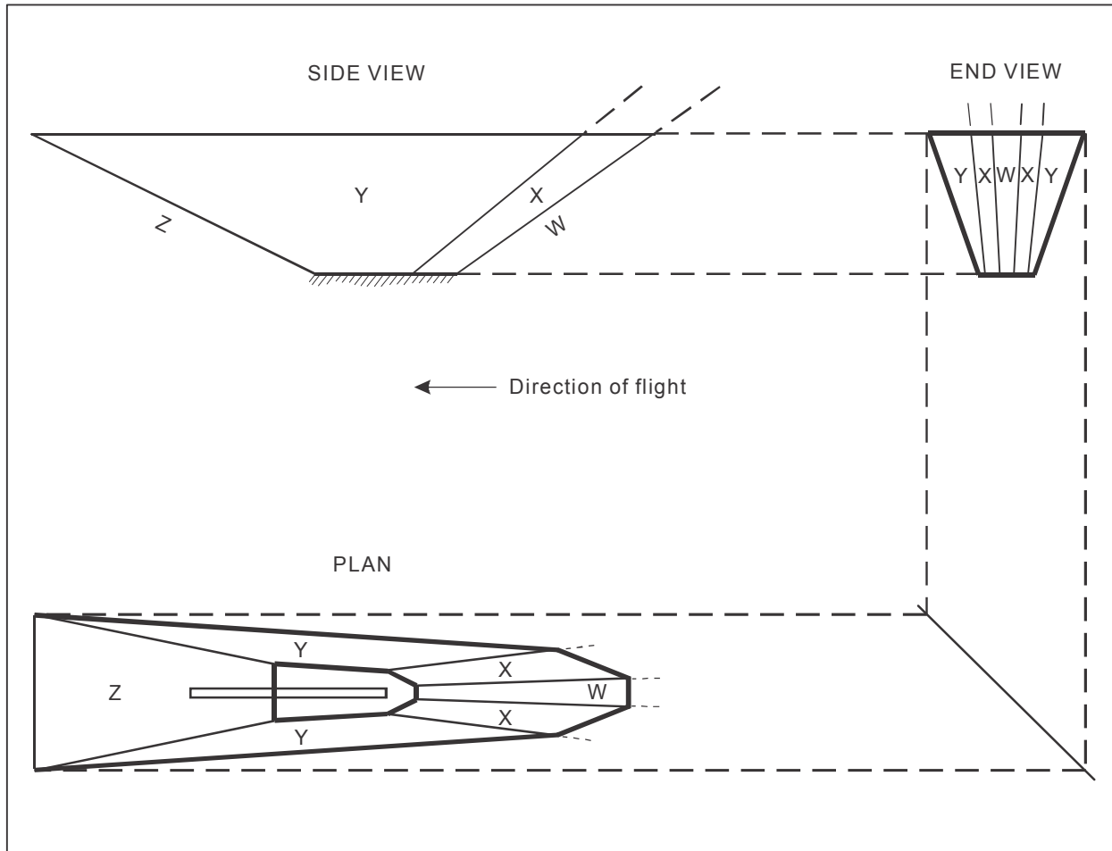
Figure III-3-6-9. Illustration of ILS obstacle assessment surfaces for GLS operations
