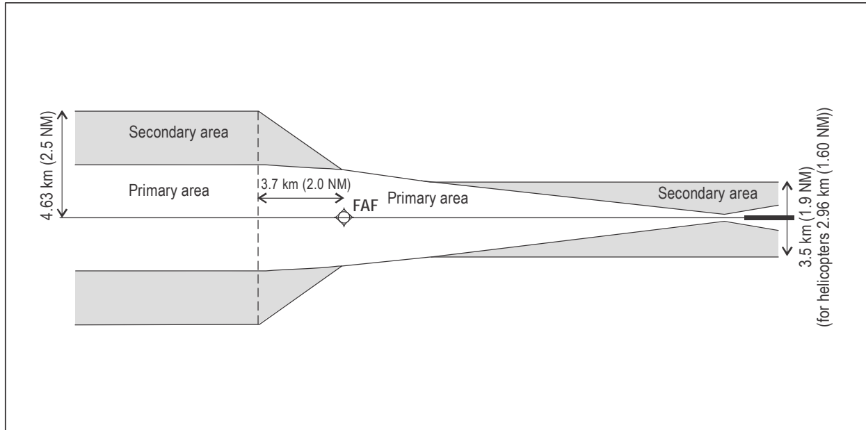
Figure III-3-5-12. Intermediate and final approach FAF far from the threshold (X surface width more than 3.5 km(1.9 NM) at FAF)
