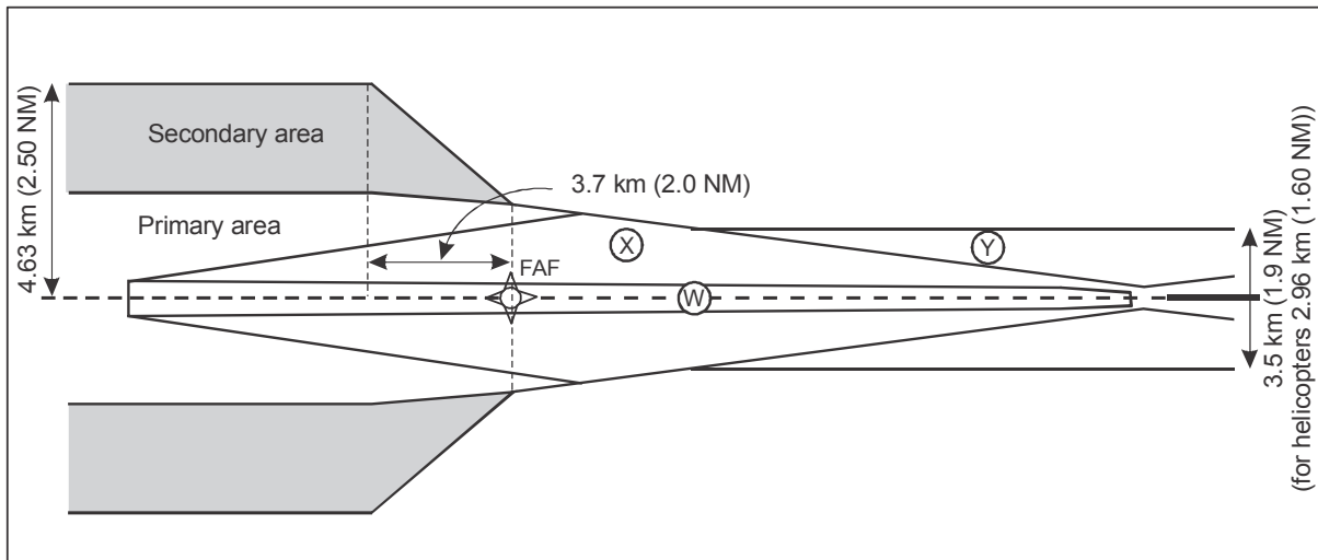
Figure III-3-5-1 a). Intermediate approach area (fully based on SBAS). FAF far from the threshold (X surface width more than 3.7 km (2.0 NM) at the FAF)
