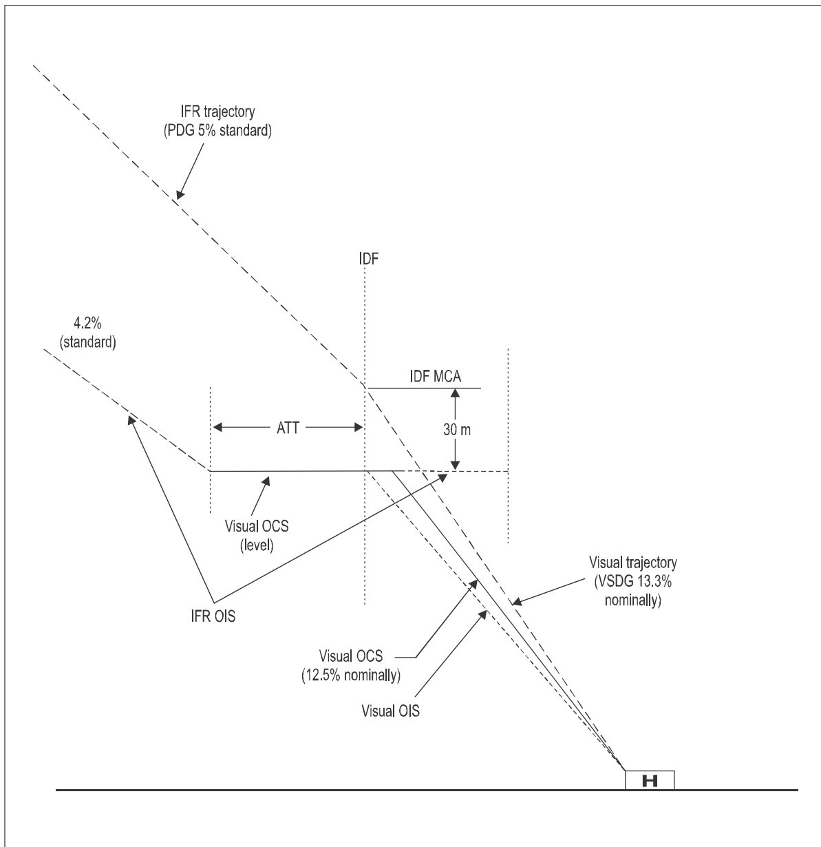
Figure IV-1-1. Vertical blending of visual segment OIS and IFR
